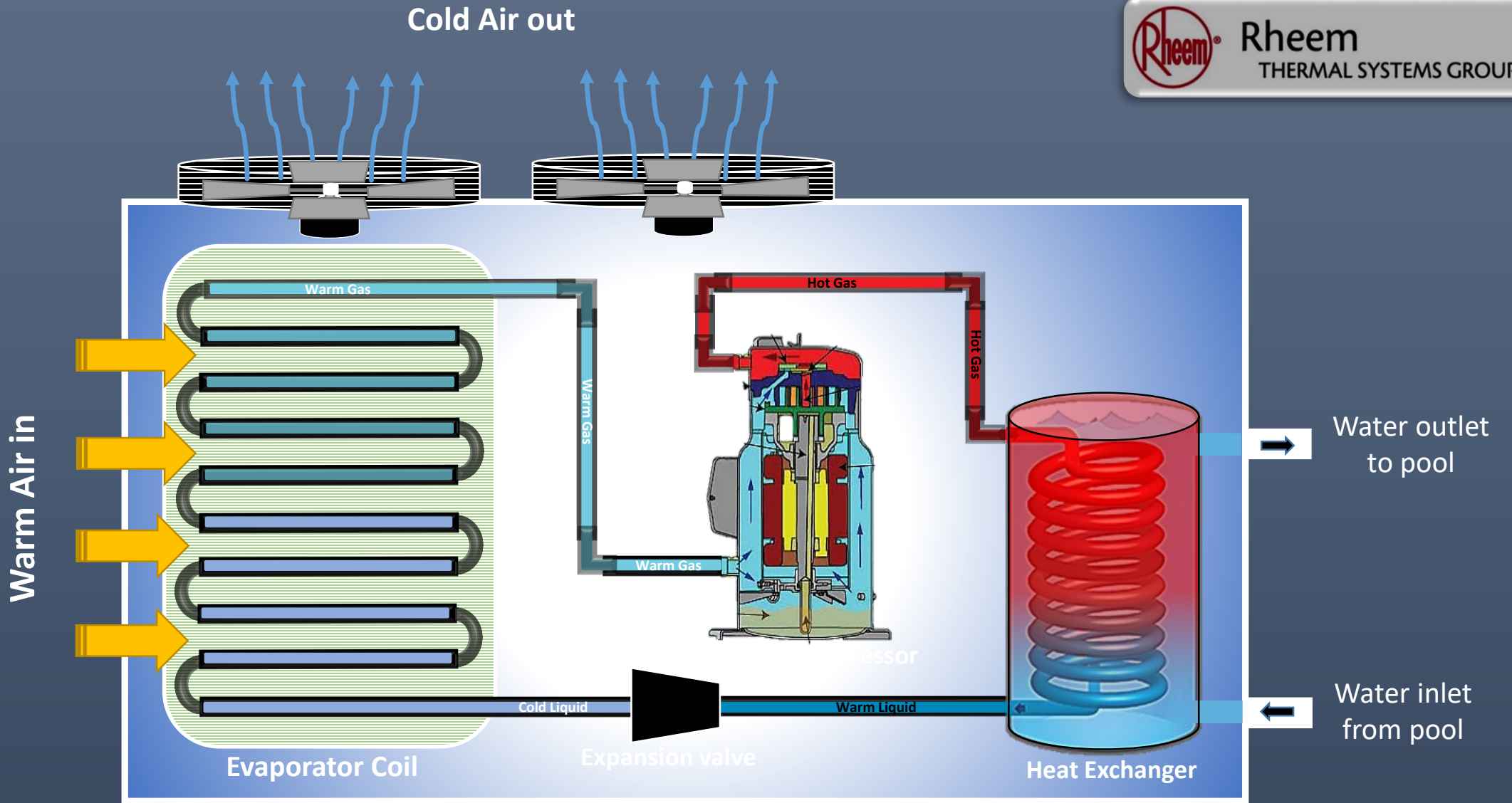
Representation of water heating process inside a Rheem Thermal pool heat pump
